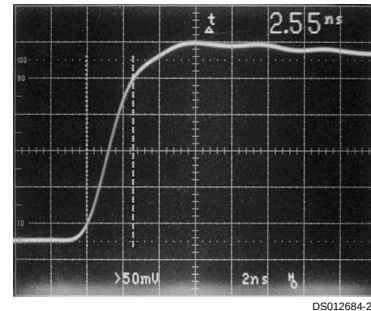
FIGURE 8. LM1283 Rise Time
